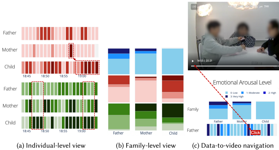
Fig. 4. Components of FamilyScope's dashboard
